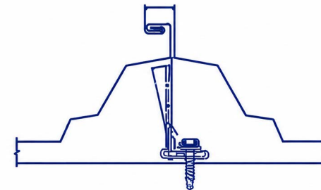
TripleLok Seam
